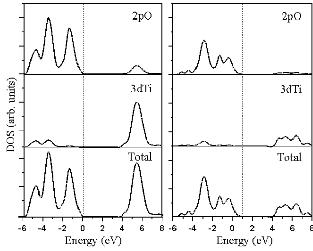
Fig. 2: The total and projected density of states for crystalline model (BST-c) (left) and asymmetric model (BST-a) (right). The zero of the energy scale was set at the Fermi energy of BST-c.
