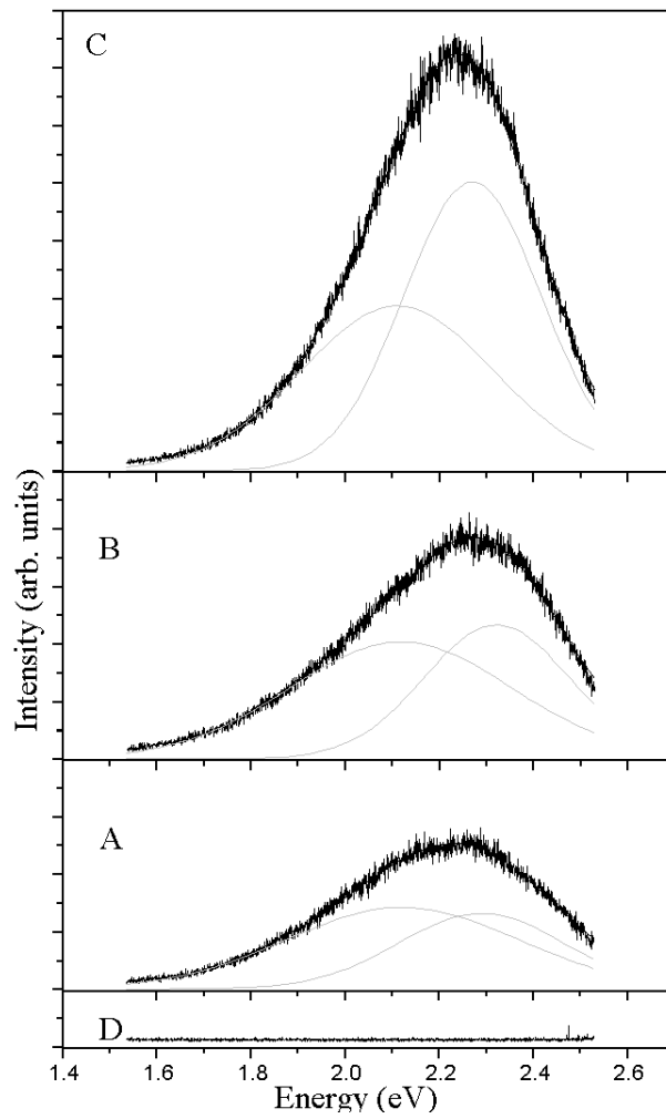
Fig. 1 : Room temperature photoluminescence spectra for (Ba,Sr)TiO 3 thin films heat treated at 300°C during (A) 2h , (B) 4h, (C) 8h and 700°C during (D) 2h.
