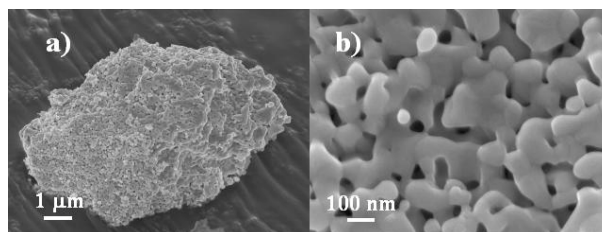
Fig 4. SEM-FEG feature of La 9.33 Si 6 O 26 powders calcined at 1000°C: a) 1 \mu m ; b) 100 nm
