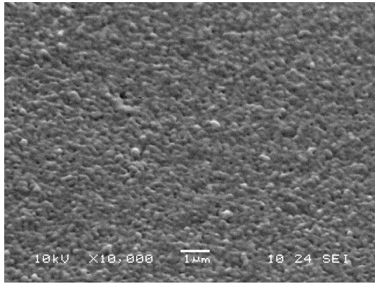
Fig. 4. SEM micrograph of PVA derived ceramics at 1200°C.
