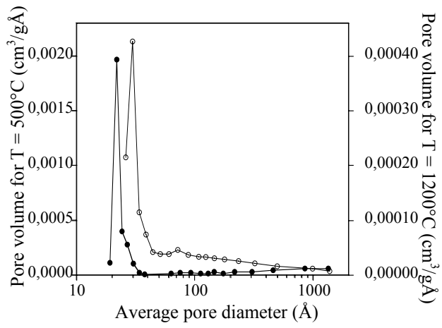
Fig. 3. Pore size distribution for albumin derived ceramics.
