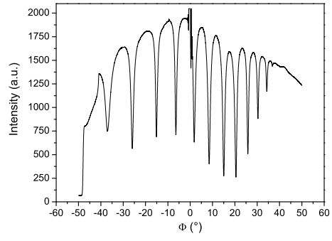
Figure 3. M-lines spectrum of a 2.08 \mu m thick pyrochlore film.
