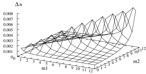
Figure 2. Index uncertainty as a function of the two mode orders.
